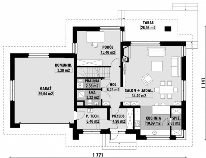
E-209 PARTER
