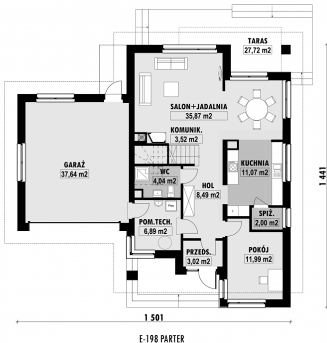
E-198 PARTER
