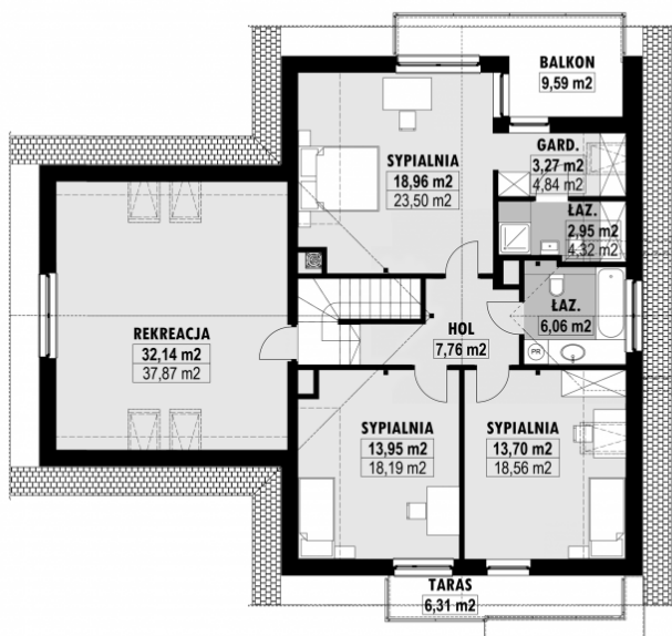
E-198 PODDASZE
