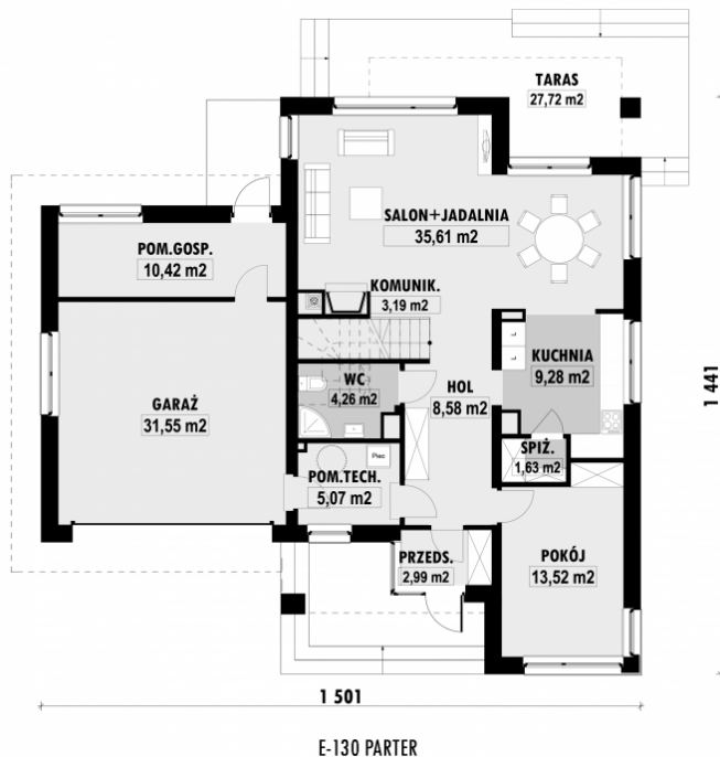
E-130 PARTER
